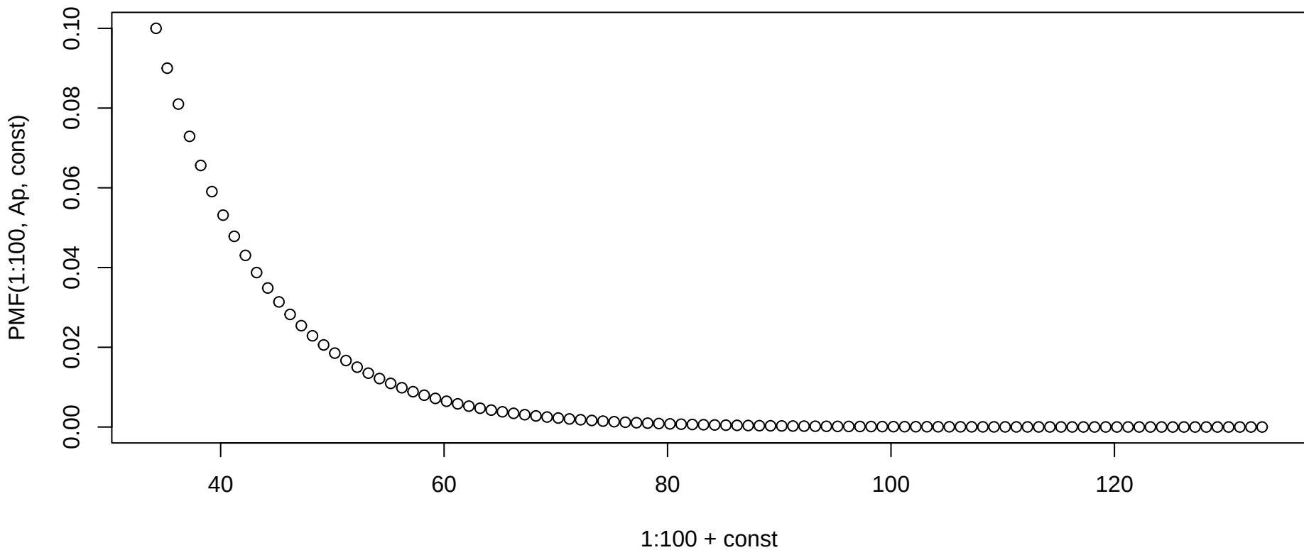
PMF of cycles for model
