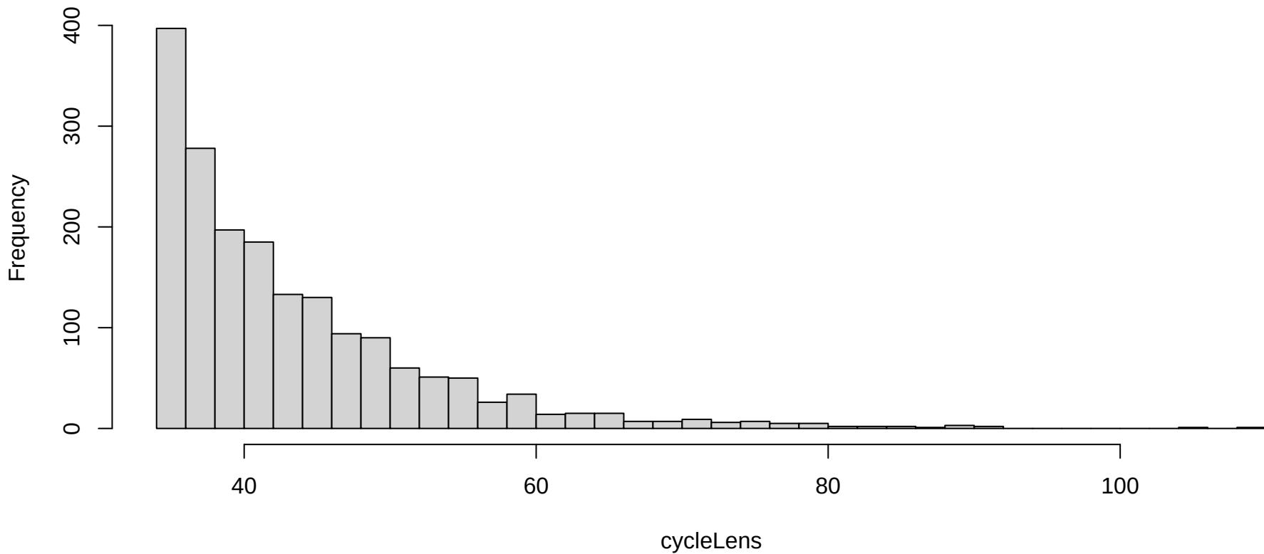
Histogram of cycleLens
